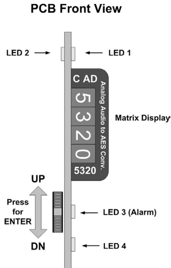
Figure 6 – Switch and Display Location
