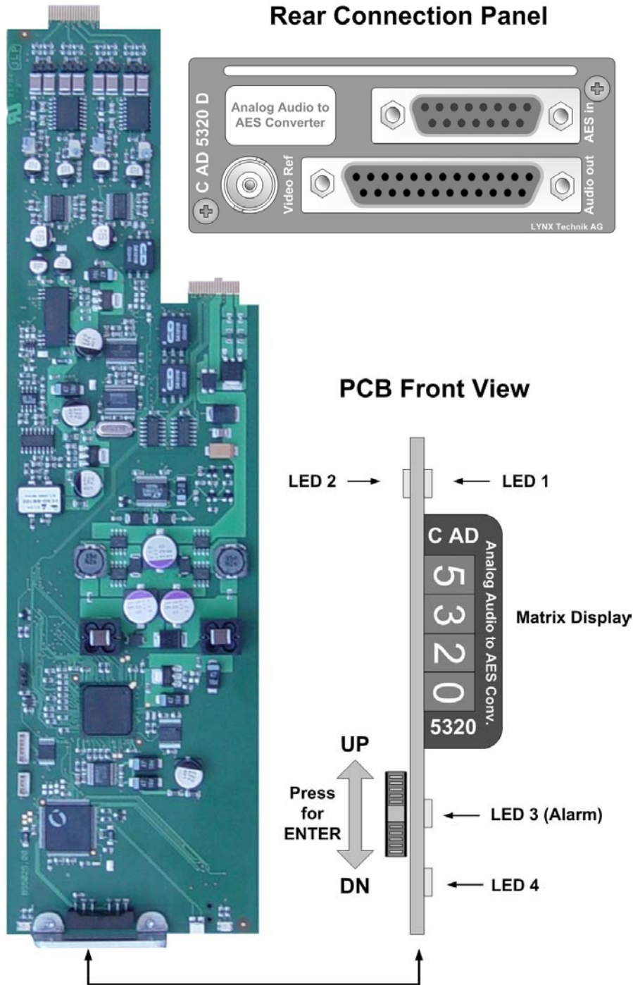
Figure 2 – Module Layout
