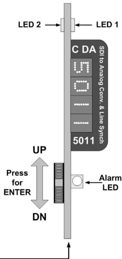
Figure 2 – Module Layout
