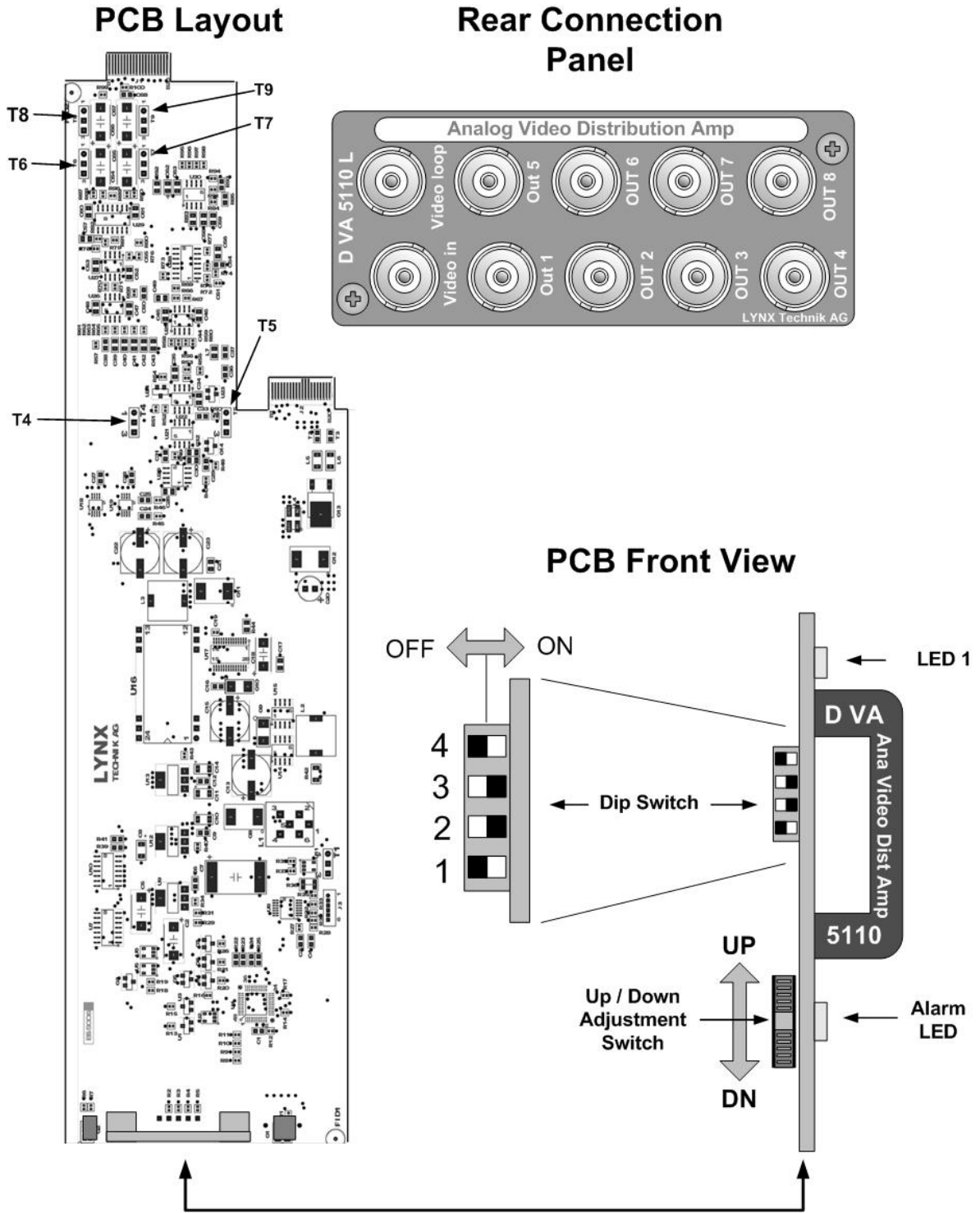
Figure 2 – Module Layout
