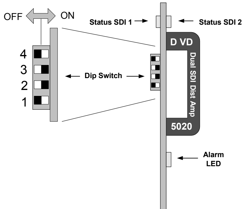
Figure 2 – Module Layout
