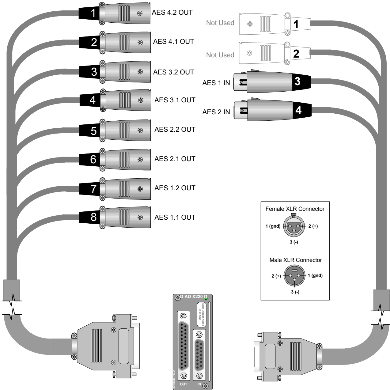
R AC M25-8 Adapter Cable
