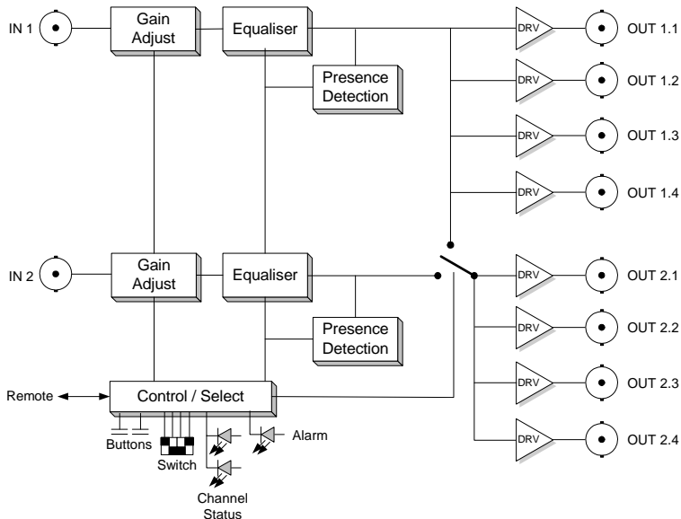
Figure 1- D VA 5720 Functional Diagram
