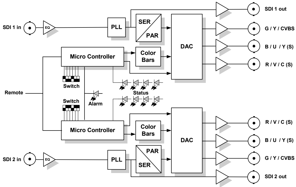
Figure 1- C DA 3002 Functional Diagram
