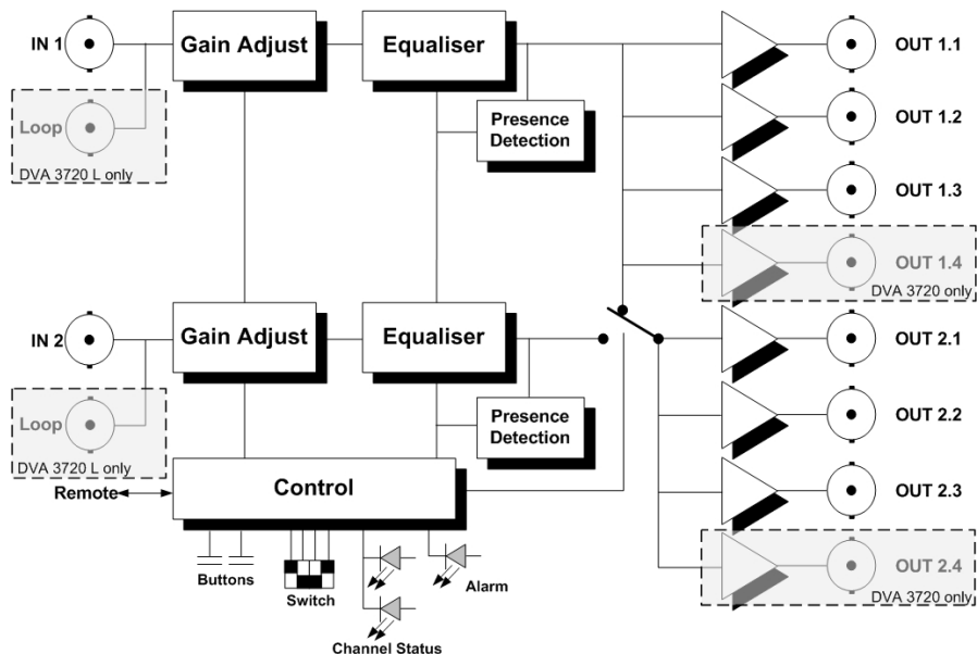
Figure 1- D VA 3720 / 3720 L Functional Diagram
