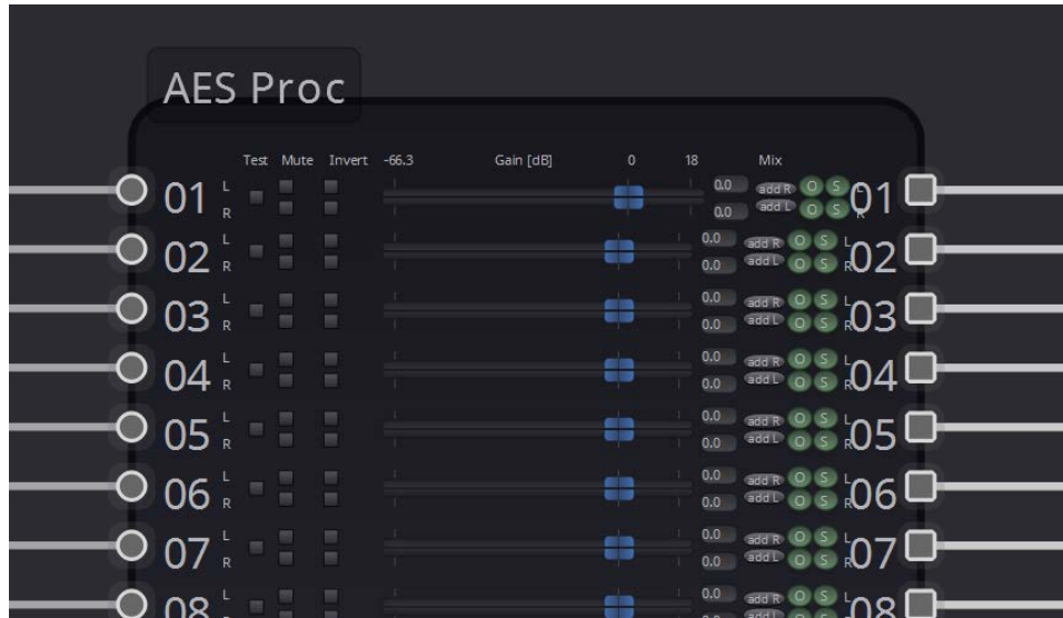
Figure 12: AES processing
