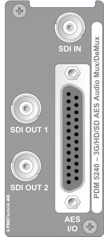
Figure 2: Rear Termination Panel P DM 5240-D
