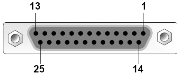
Figure 6: SubD25 Audio connector (looking into connector from back of module)
