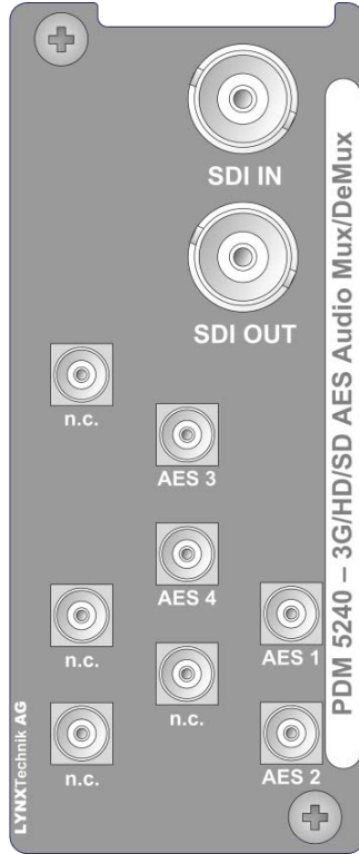
Figure 3: Rear Termination Panel P DM 5240-U
