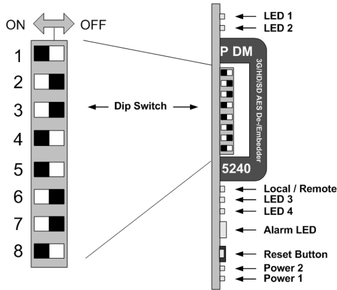
Figure 7: Card Edge switches and LED positions
