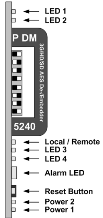
Figure 8: Card Edge LEDs
