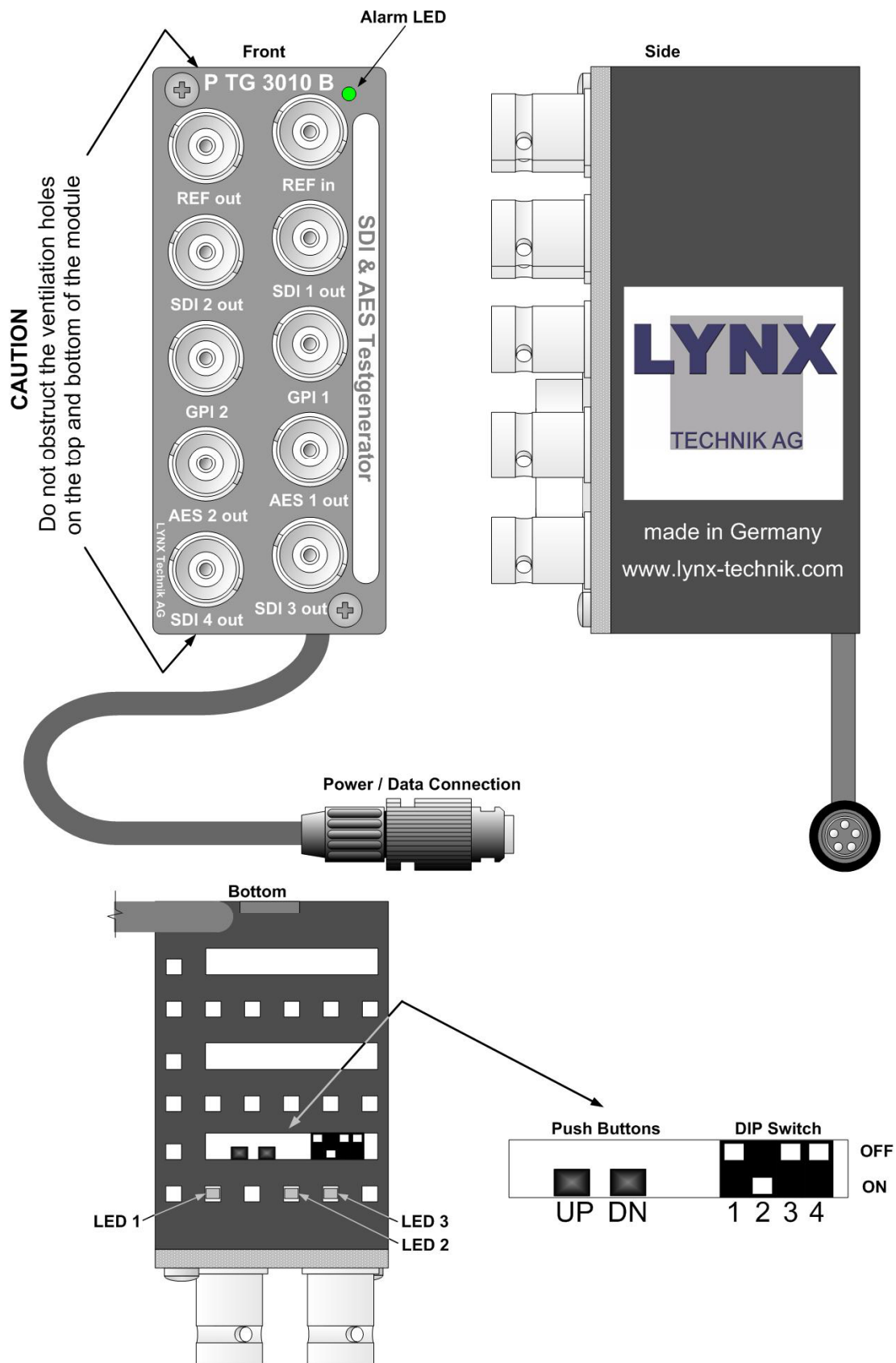
Fig.2: Physical Layout P TG 3010 B
