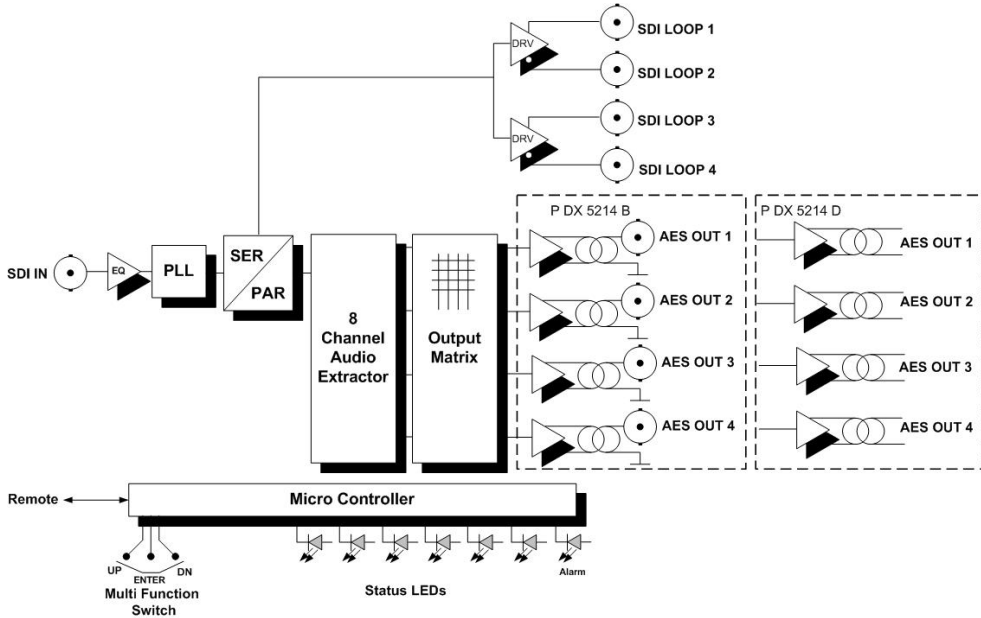
Figure 1- P DX 5214 D Functional Diagram
